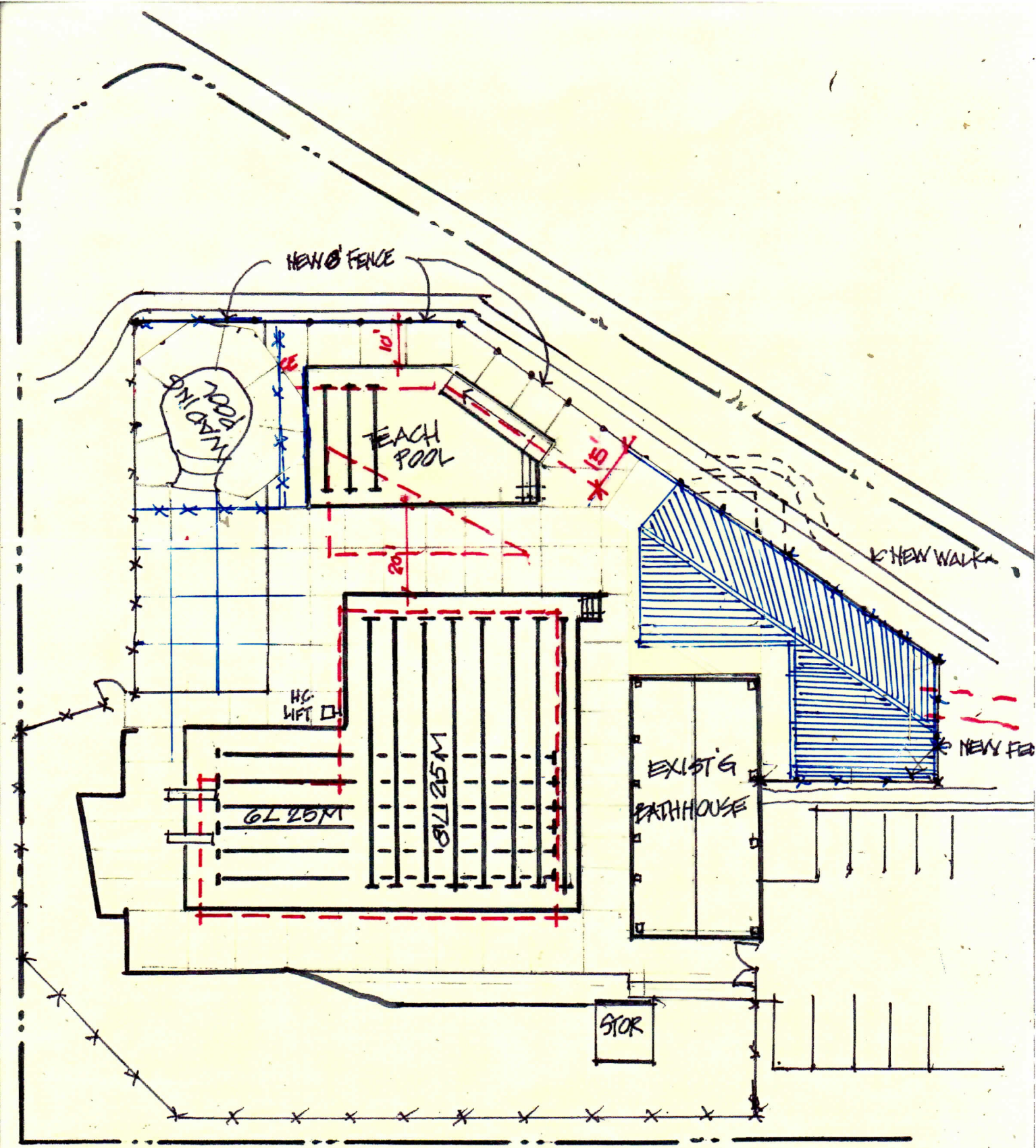
SCHEME 4 1" = 30'-0" 5/29/15 THREE FILTERS
